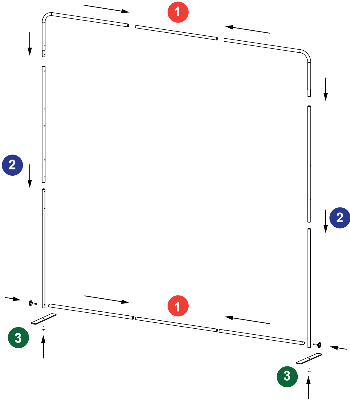
Frame Assembly
