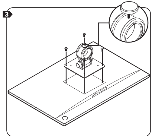
Lock VESA behind the screen
