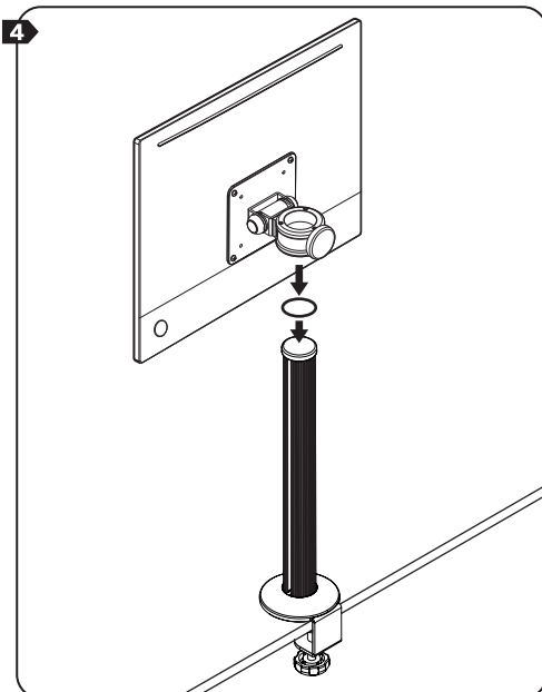
Place rubber ring at desired height
